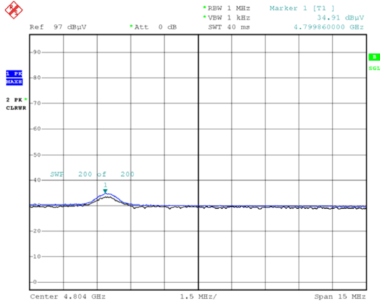
Radiated Spurious Emissions plot – Average Reading (GFSK, Ch.0 2nd Harmonic, X-V)
