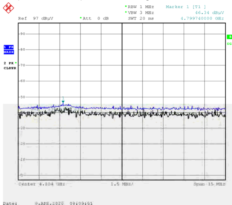
Radiated Spurious Emissions plot – Peak Reading (GFSK, Ch.0 2nd Harmonic, X-V)
