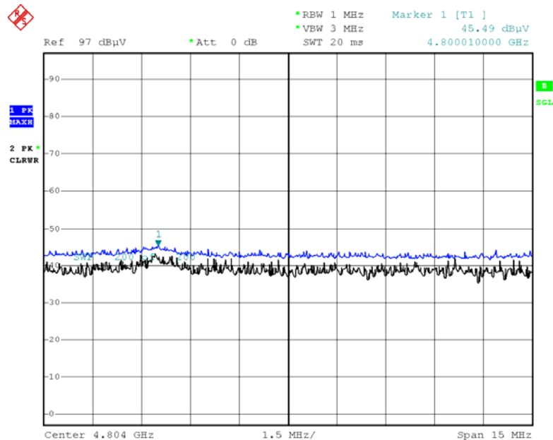
Radiated Spurious Emissions plot – Peak Reading (8DPSK, Ch.0 2nd Harmonic, V)
