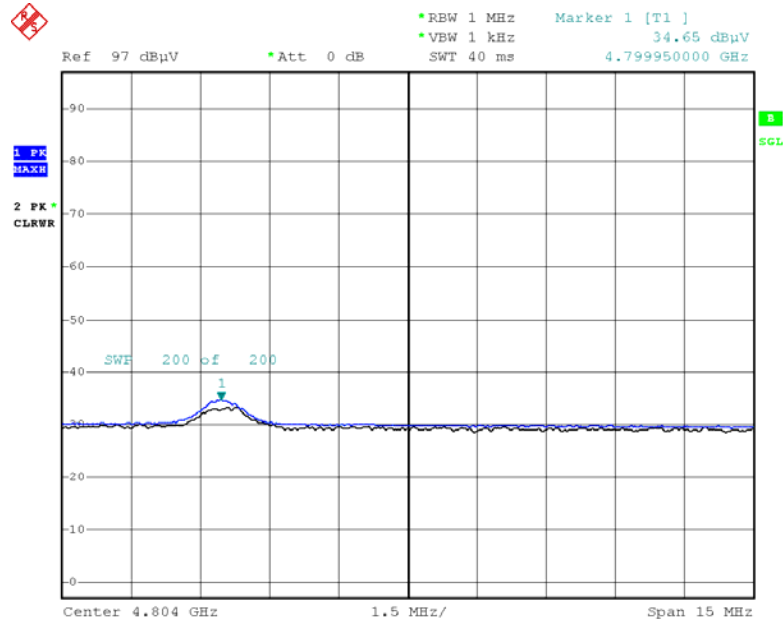
Radiated Spurious Emissions plot – Average Reading ( \pi/4 DQPSK, Ch.0 2nd Harmonic, V)
