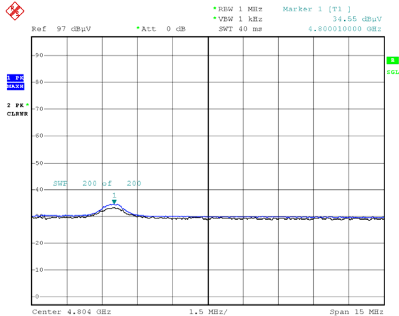
Radiated Spurious Emissions plot – Average Reading (8DPSK, Ch.0 2nd Harmonic, V)
