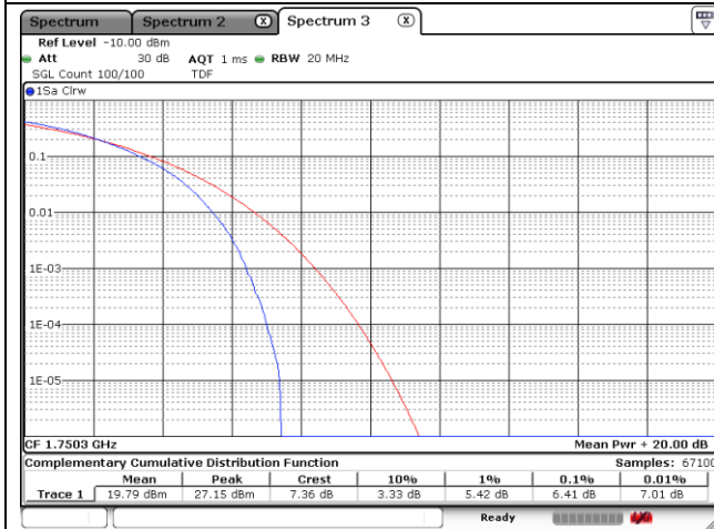
10 MHz + 20 MHz 64QAM Middle Channel - Full RB
