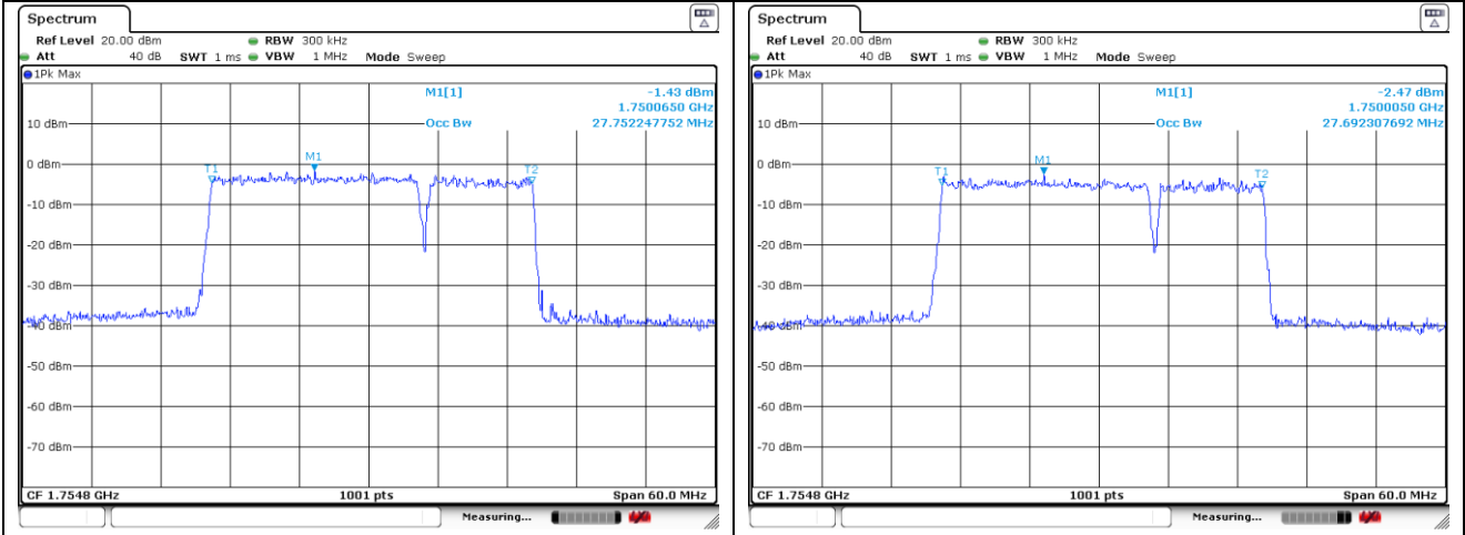
20 MHz + 10 MHz QPSK Middle Channel - Full RB
