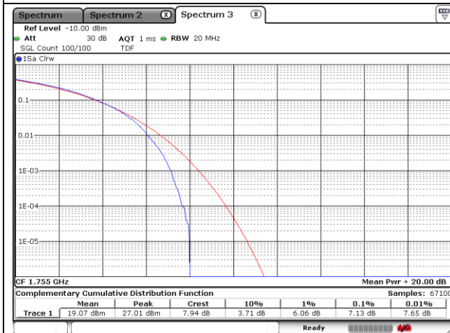
15 MHz + 15 MHz 64QAM Middle Channel - Full RB
