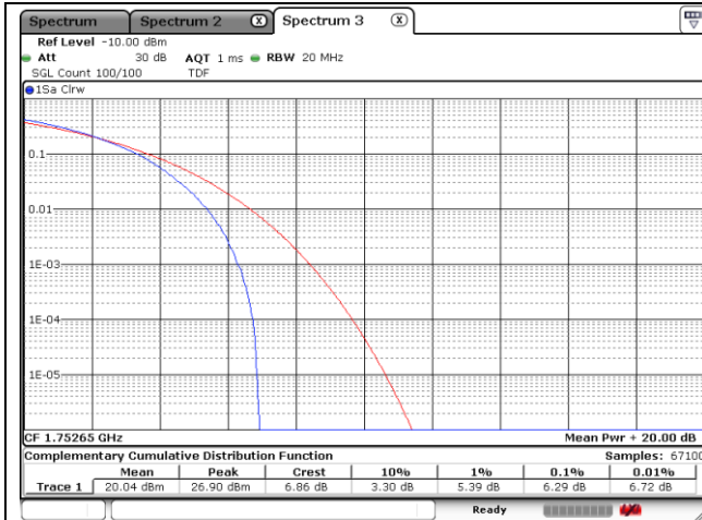
10 MHz + 15 MHz 64QAM Middle Channel - Full RB
