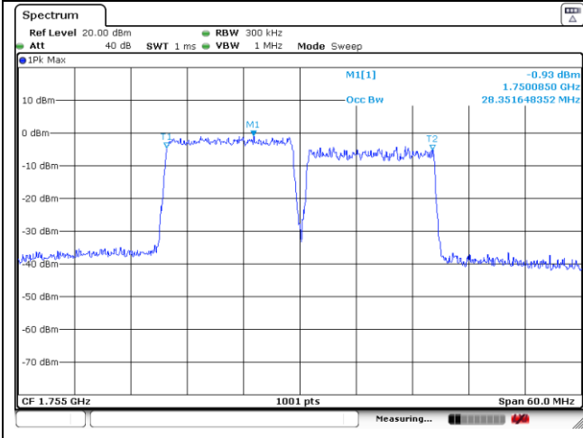
15 MHz + 15 MHz QPSK Middle Channel - Full RB
