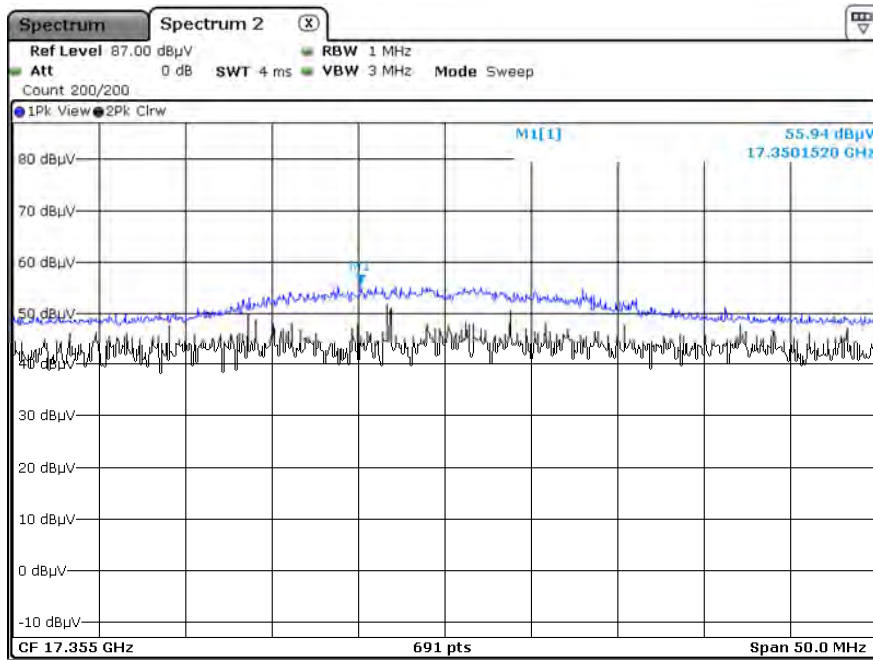
Peak Reading (802.11a, Ch.157 3rd Harmonic, X-H)
