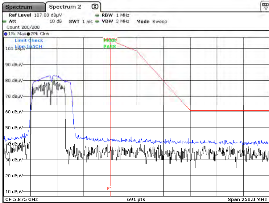
Peak Reading (802.11ac_VHT40, Ch.159, X-V)
