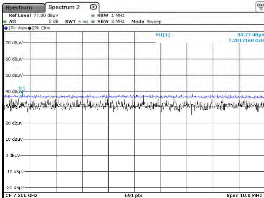
Radiated Spurious Emissions plot – Peak Reading (GFSK, Ch. 0 3rd Harmonic, X-V)
