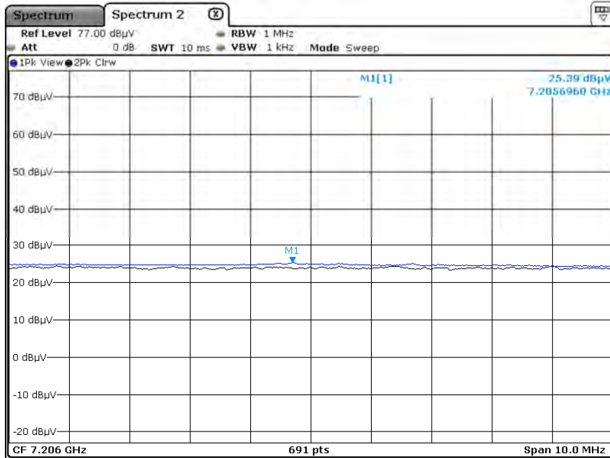
Radiated Spurious Emissions plot – Average Reading (GFSK, Ch. 0 3rd Harmonic, X-V)
