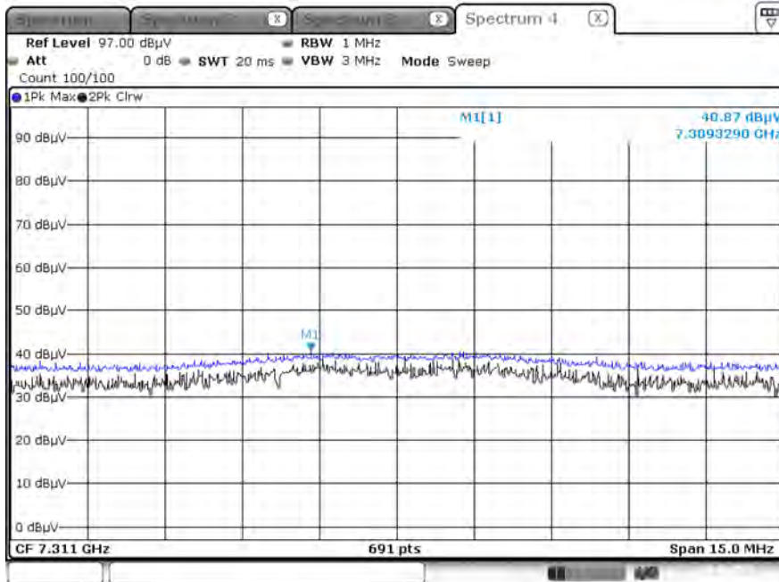
Radiated Spurious Emissions plot – Peak Reading (802.11b, Ch.6 3rd Harmonic, X-V)
