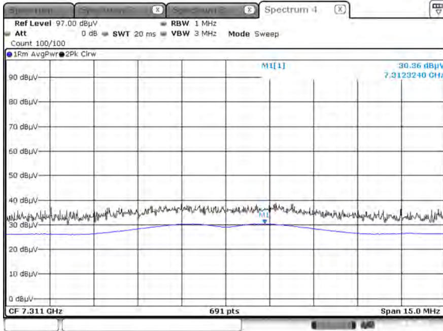
Radiated Spurious Emissions plot – Average Reading (802.11b, Ch.6 3rd Harmonic, X-V)
