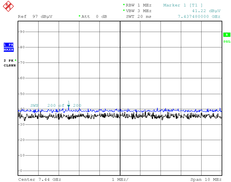
Radiated Spurious Emissions plot – Peak Result (8DPSK, Ch.78 3rd Harmonic, X-V)
