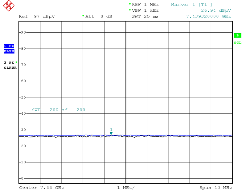
Radiated Spurious Emissions plot – Average Result (8DPSK, Ch.78 3rd Harmonic, X-V)
