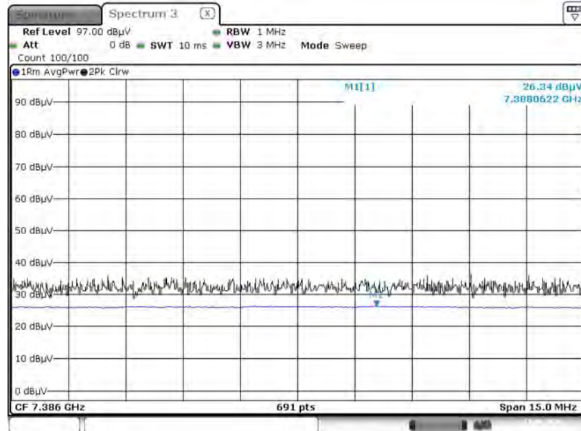
Radiated Spurious Emissions plot – Average Reading (802.11g, Ch.11 3rd Harmonic, X-V)
