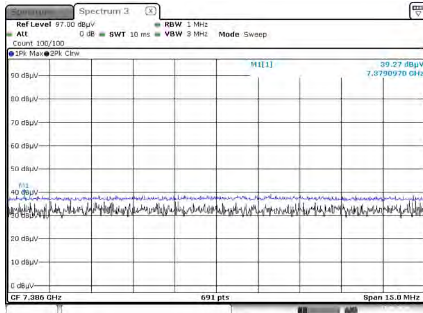
Radiated Spurious Emissions plot – Peak Reading (802.11g, Ch.11 3rd Harmonic, X-V)
