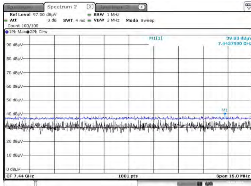
Radiated Spurious Emissions plot – Average & Peak Reading ( \pi/4 DQPSK, Ch.78 3rd Harmonic, X-H)
