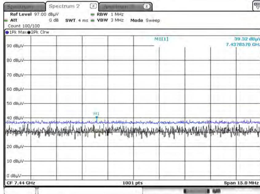
Radiated Spurious Emissions plot – Average & Peak Reading (GFSK, Ch.78 3rd Harmonic, X-H)
