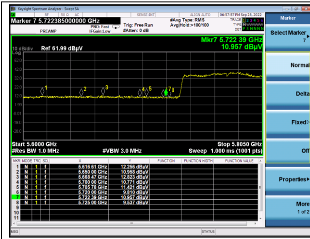
Middle channel Band edge (Peak) - Band 3
