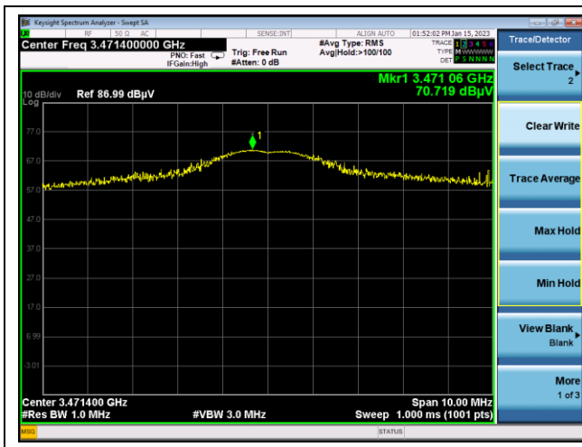
8 th harmonic
