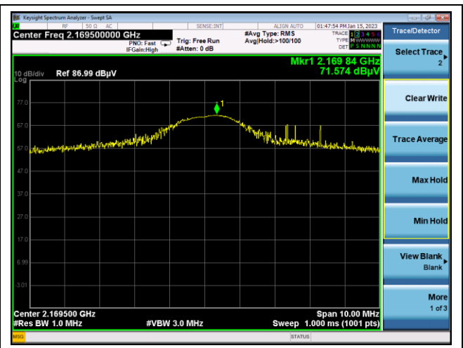
5 th harmonic
