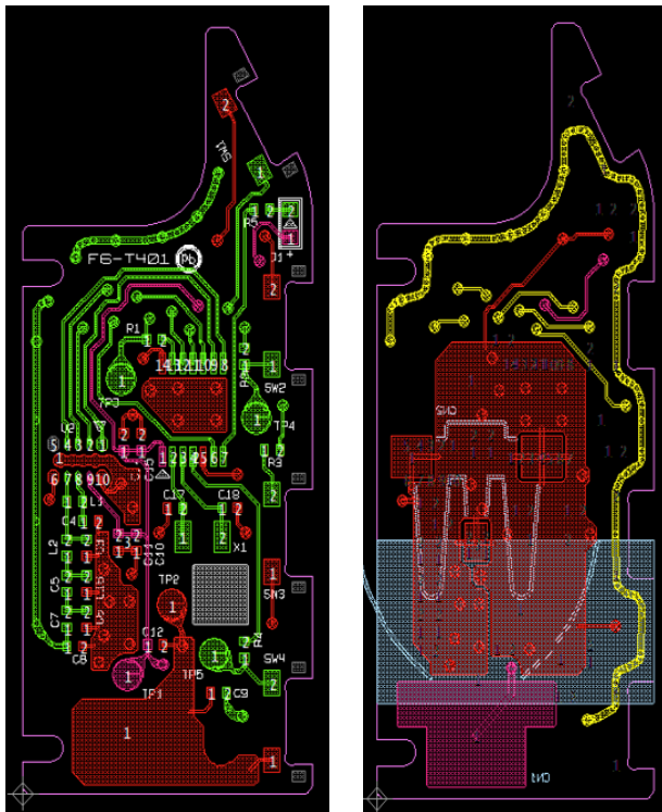
PCB PATTERN DIAGRAM
