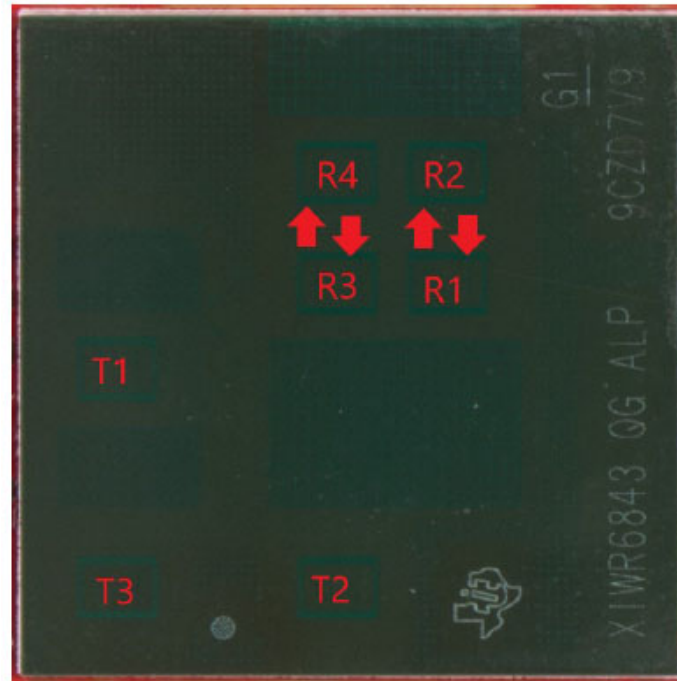
Figure 2. Antenna Picture
