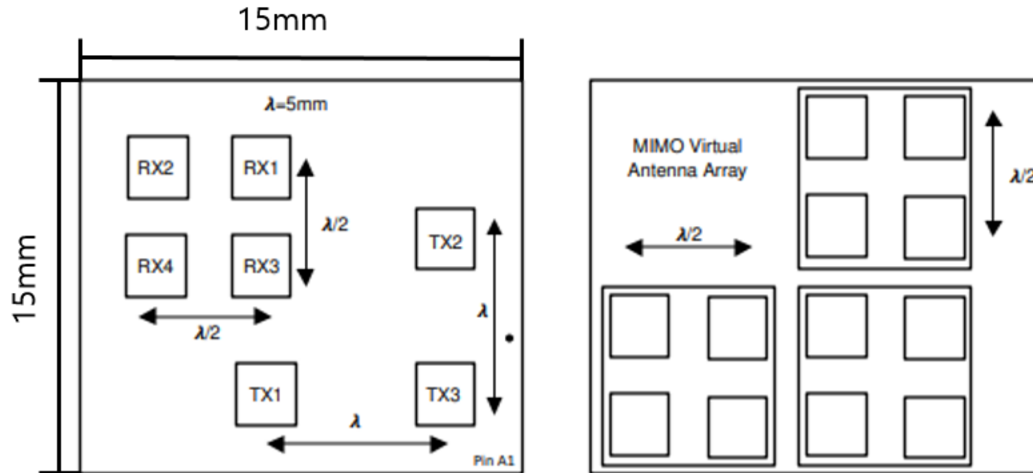
Figure 1. Antenna Positions (Placement and Relative Spacing)
