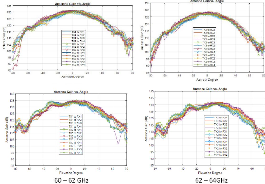
Figure 3. Antenna Radiation pattern
