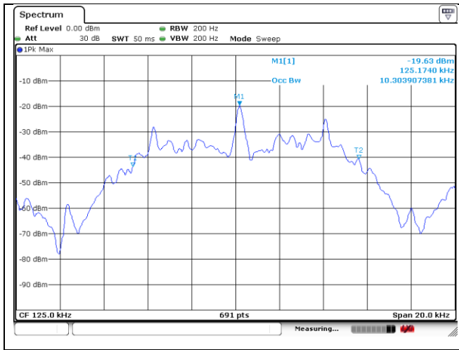
DRV Antenna
