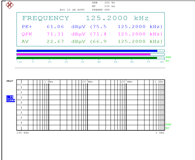
INT1 Antenna
