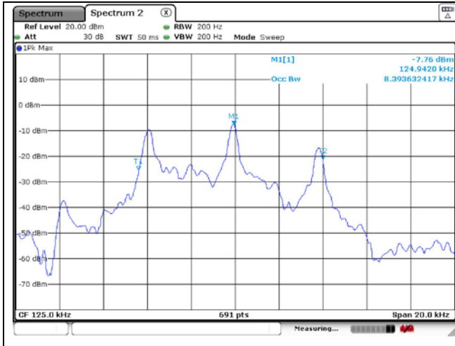
REAR Antenna
