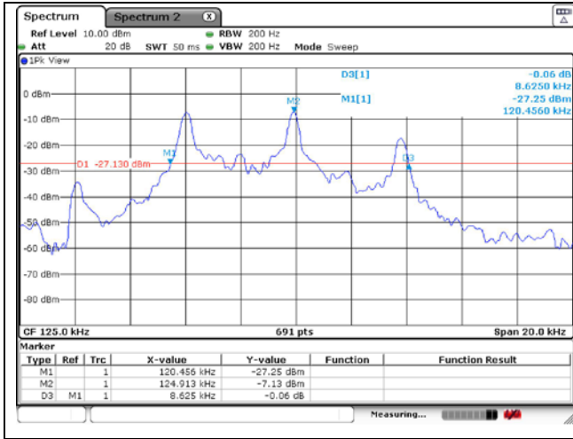
REAR Antenna
