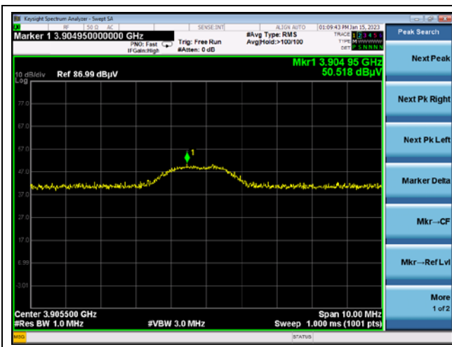
9 th harmonic
