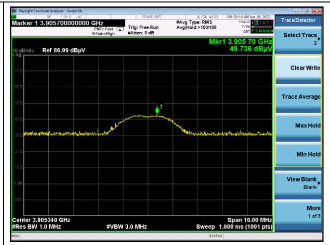
9 th harmonic
