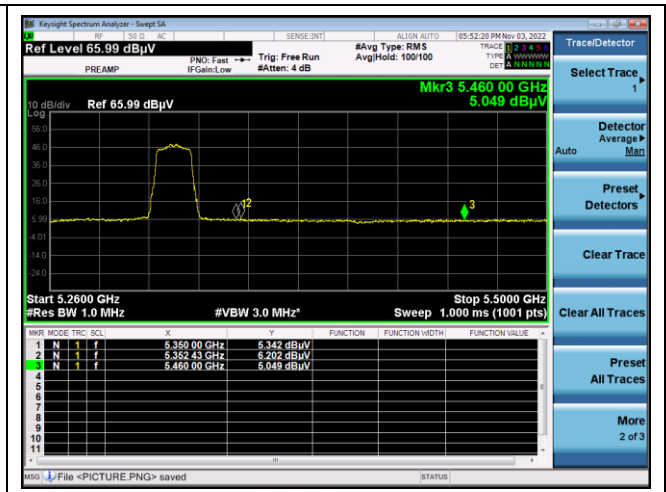
High channel Band edge (Average) - Band 2A
