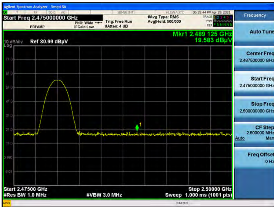
Radiated Restricted Band Edges plot – Peak Reading ( \pi/4 DQPSK, Ch.78, X-V)
