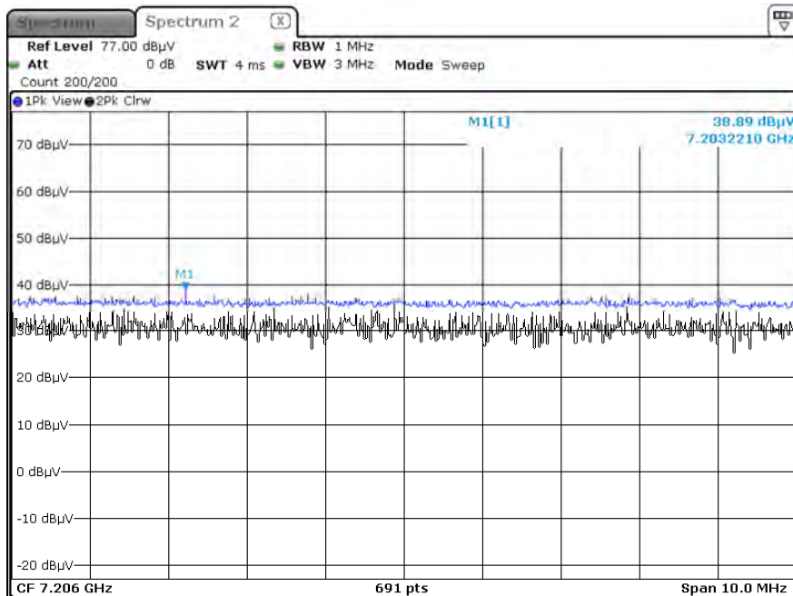
Radiated Spurious Emissions plot – Peak Reading ( \pi/4 DQPSK, Ch.0 3rd Harmonic, X-H)
