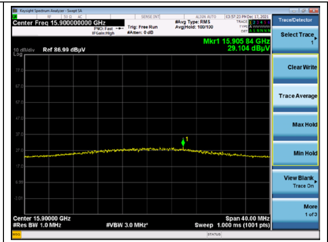
Middle channel 3 rd harmonic (Average) - Band 2A
