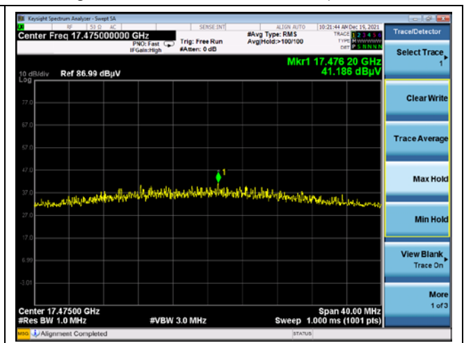
High channel 3 rd harmonic (Peak) - Band 3
