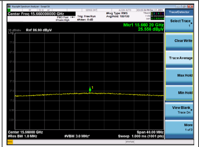
Middle channel 3 rd harmonic (Average) - Band 1
