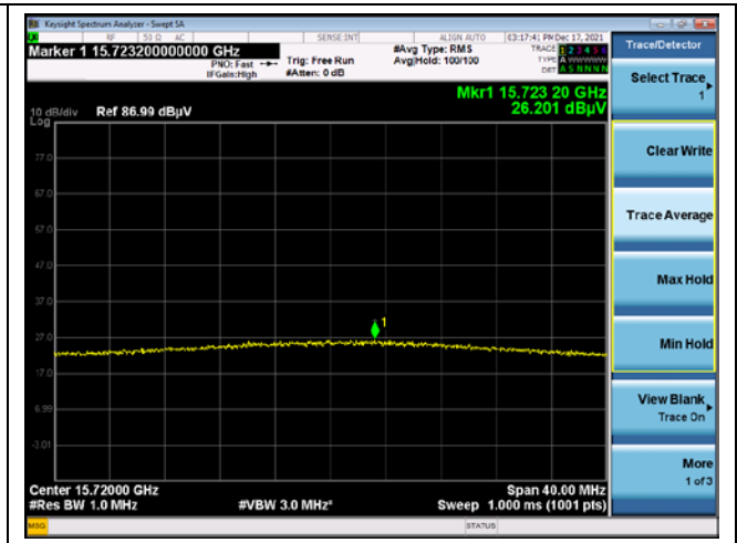
High channel 3 rd harmonic (Average) - Band 1
