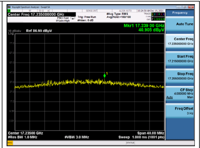
Low channel 3 rd harmonic (Peak) - Band 3
