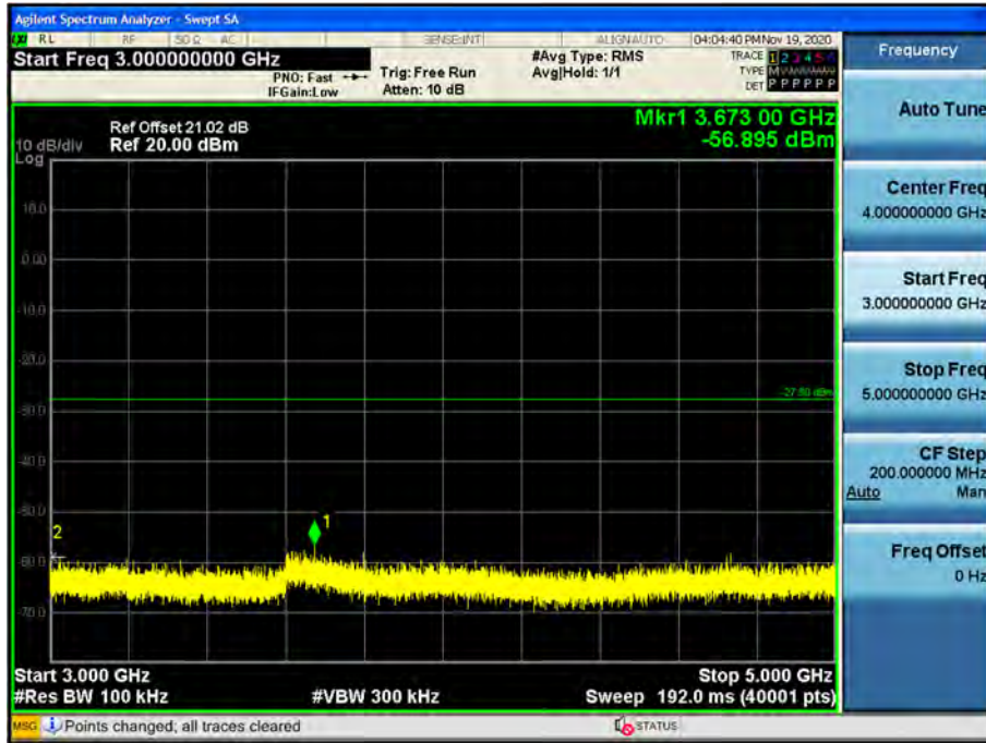
Conducted Spurious Emission (802.11n_HT20_Ch.1_MCS0)
