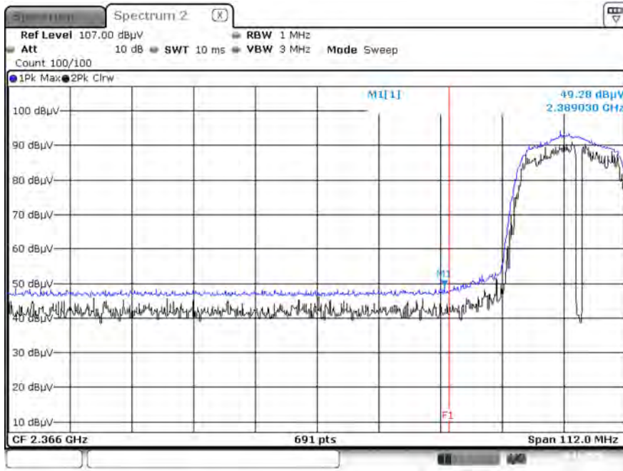
Radiated Restricted Band Edges plot – Peak Reading (802.11n(HT20), Ch.1, X-V)
