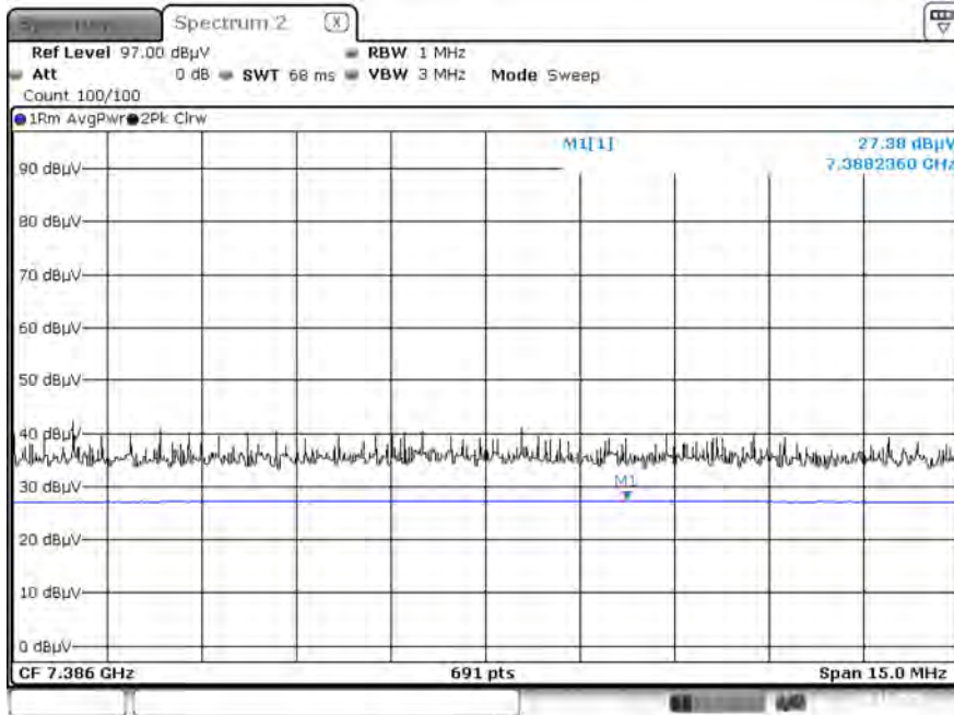
Radiated Spurious Emissions plot – Average Reading (802.11g, Ch.11 3rd Harmonic)
