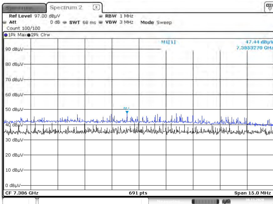
Radiated Spurious Emissions plot – Peak Reading (802.11g, Ch.11 3rd Harmonic)
