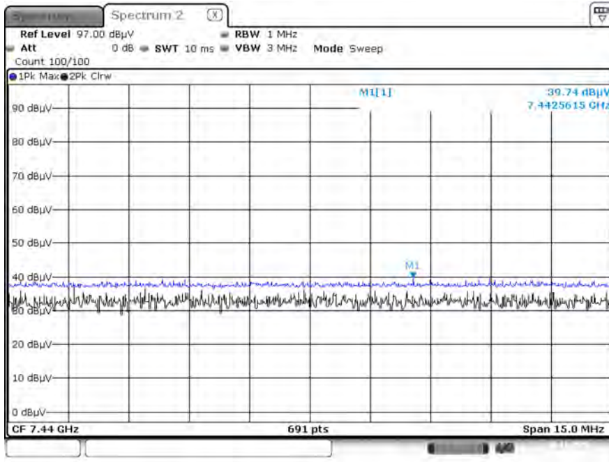
Radiated Spurious Emissions plot – Peak Reading ( \pi/4 DQPSK, Ch.78 3rd Harmonic, X-H)
