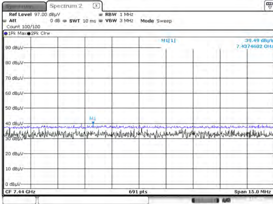
Radiated Spurious Emissions plot – Average Reading (GFSK, Ch.78 3rd Harmonic, X-H)
