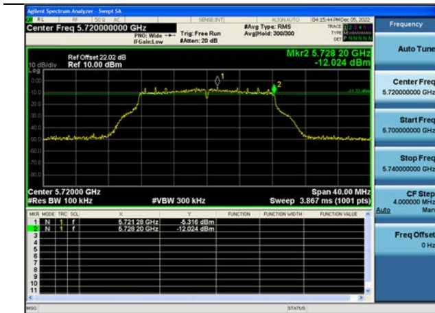
802.11ac_VHT20 CH.144
