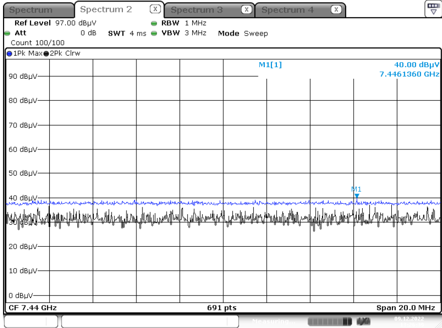
Radiated Spurious Emissions plot – Average & Peak Result (8DPSK, Ch.78 3rd Harmonic, X-H)
