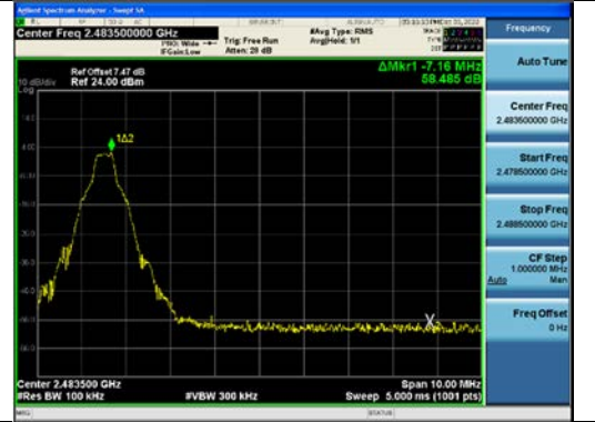
8DPSK(without hopping) Band Edge(CH.78)
