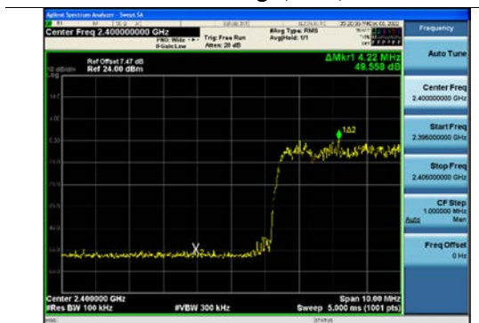
\pi/4 DQPSK(with hopping) Band Edge(CH.0)
