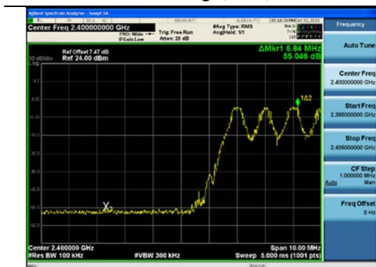
8DPSK(with hopping) Band Edge(CH.0)
