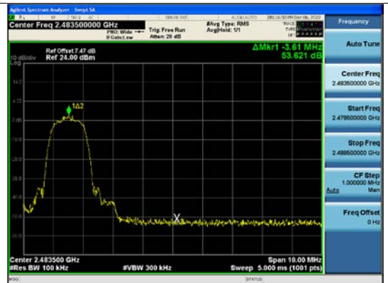
\pi/4 DQPSK (without hopping) Band Edge(CH.78)
