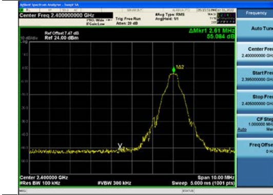
8DPSK(without hopping) Band Edge(CH.0)
