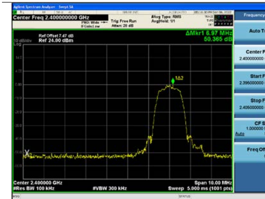
\pi/4 DQPSK(without hopping) Band Edge(CH.0)
