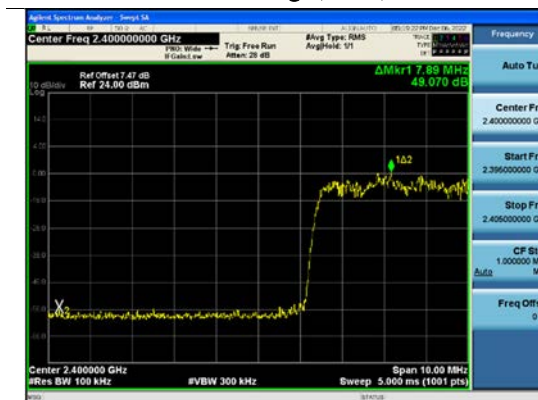
\pi/4 DQPSK(with hopping) Band Edge(CH.0)
