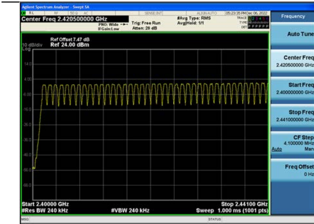
8DPSK Number of Channels (2.4 GHz - 2.441 GHz)
