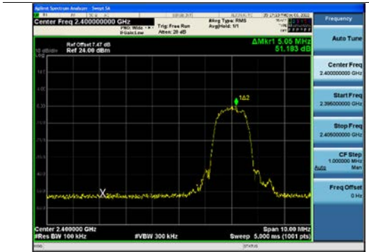
\pi/4 DQPSK(without hopping) Band Edge(CH.0)
