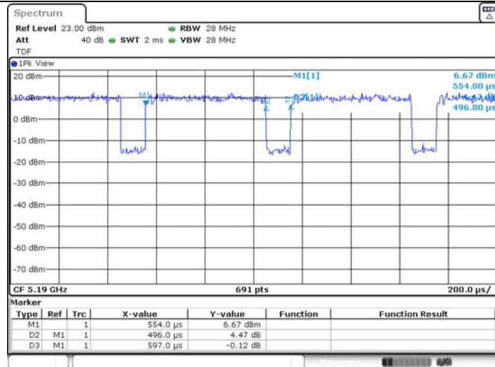
802.11ac_VHT40
