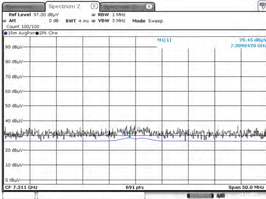
Radiated Spurious Emissions plot – Average Result (802.11b, Ch.6 3rd Harmonic)
