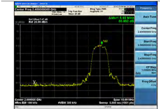
\pi/4 DQPSK(without hopping) Band Edge(CH.0)
