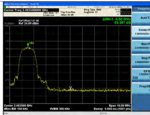
\pi/4 DQPSK (without hopping) Band Edge(CH.78)
