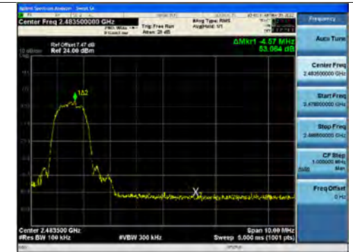
\pi/4 DQPSK (without hopping) Band Edge(CH.78)
