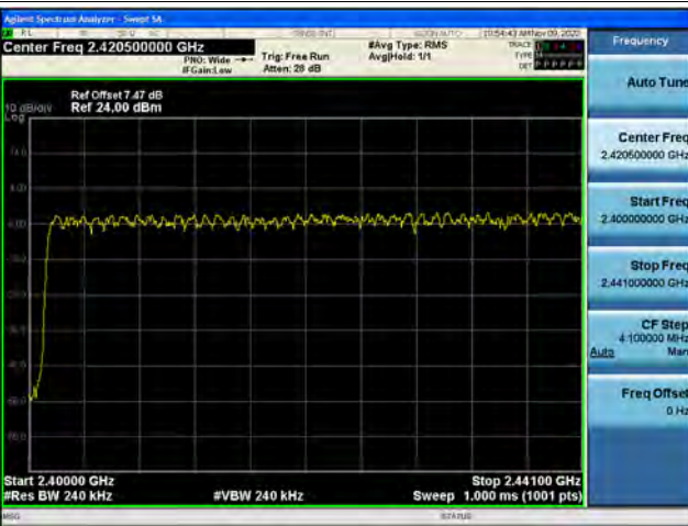
\pi/4 DQPSK Number of Channels (2.4 GHz - 2.441 GHz)
