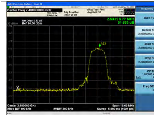
\pi/4 DQPSK(without hopping) Band Edge(CH.0)
