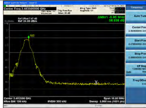
8DPSK(without hopping) Band Edge(CH.78)
