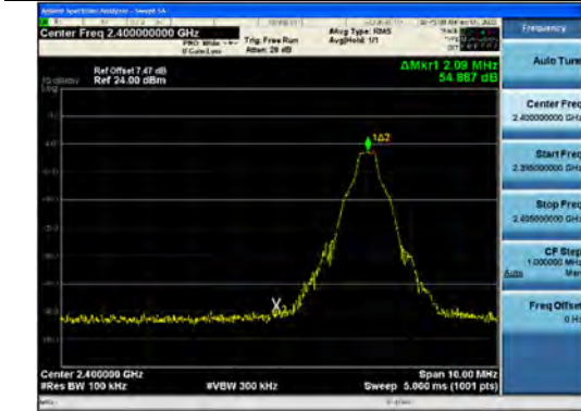
8DPSK(without hopping) Band Edge(CH.0)
