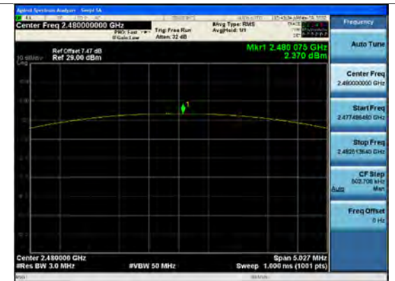
GFSK : Peak Power (CH.78)
