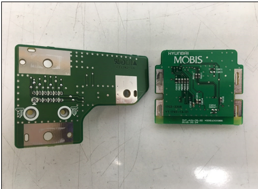
Bottom view of Sub PCB3
