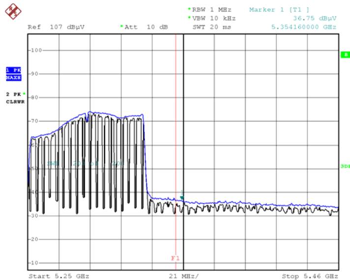
Average Reading (802.11 ac_VHT80_MCS0, Ch.58, X-V)
