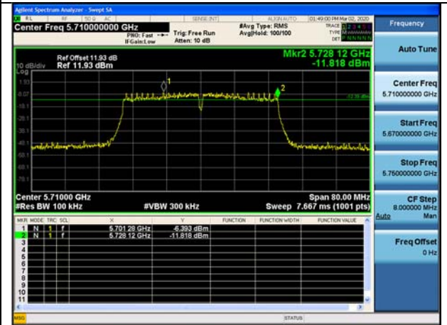
802.11ac_VHT40 CH.142
