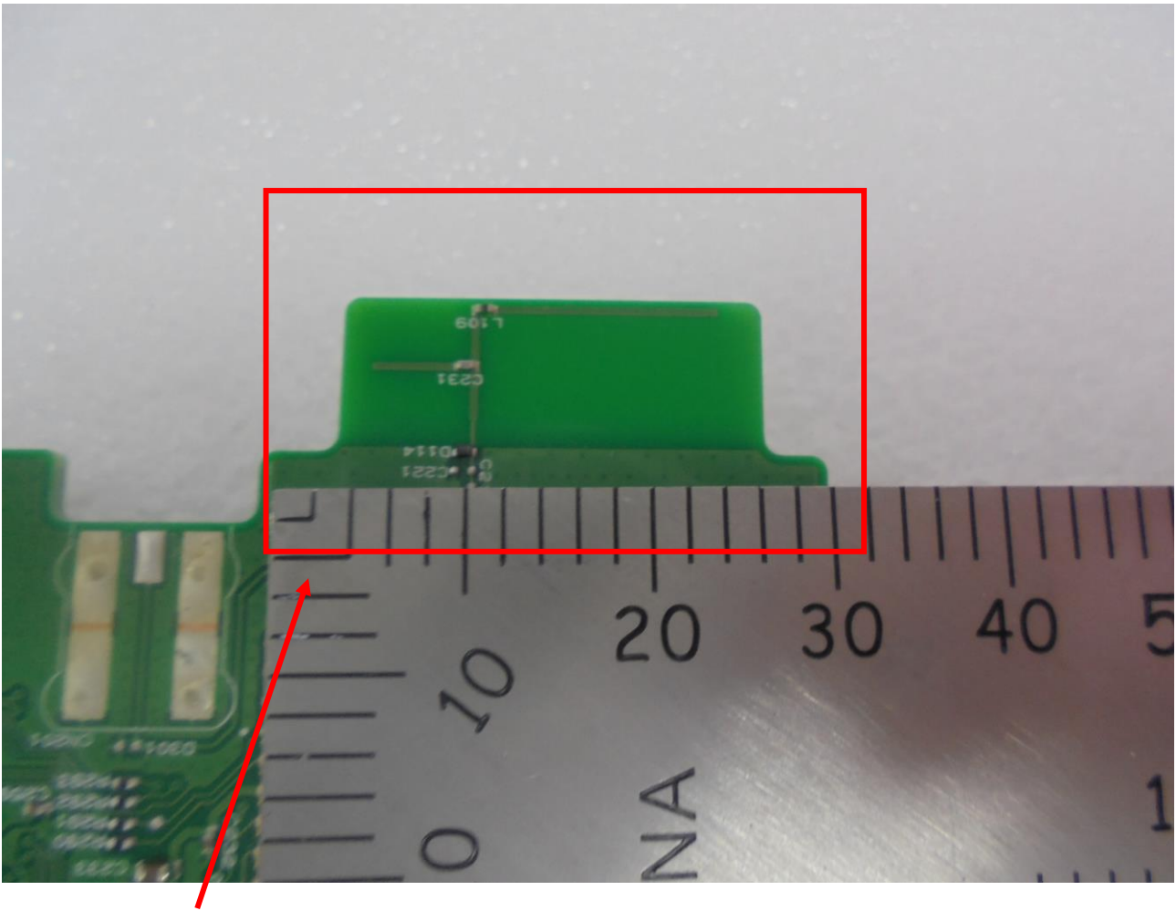
WIFI Antenna
