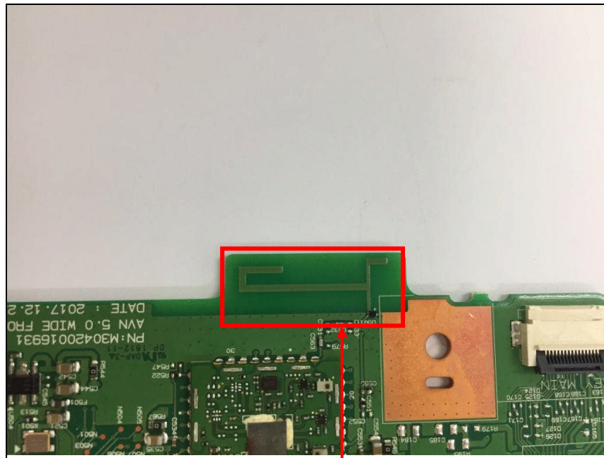
Wi-Fi Pattern Antenna
