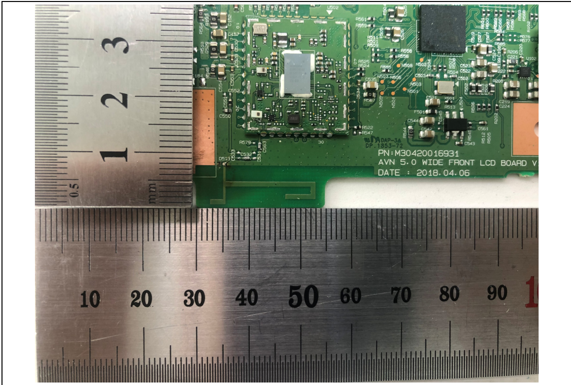
<Wifi Antenna>
