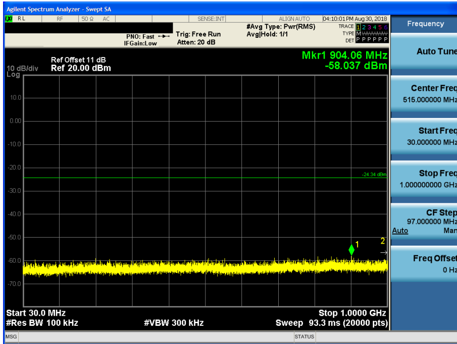
Conducted Spurious Emission (802.11n_Ch.1_5 Mbps)
