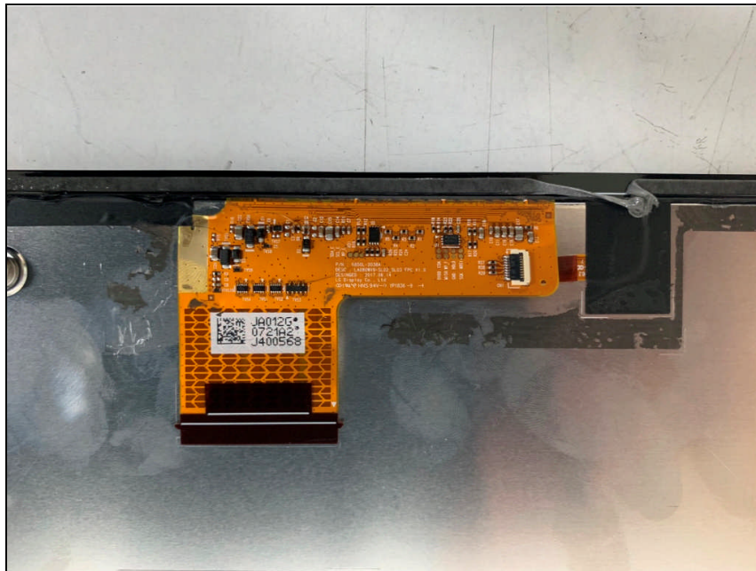
Bottom view of Sub FPCB1
