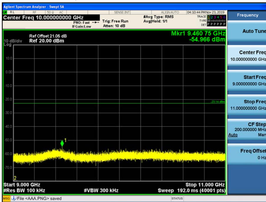
Conducted Spurious Emission (802.11_n(20M)_Ch.1_6.5 Mbps)
