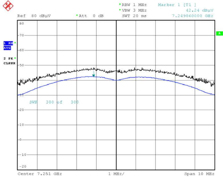
Radiated Spurious Emissions plot – Average Reading (802.11b, Ch.2 3rd Harmonic)
