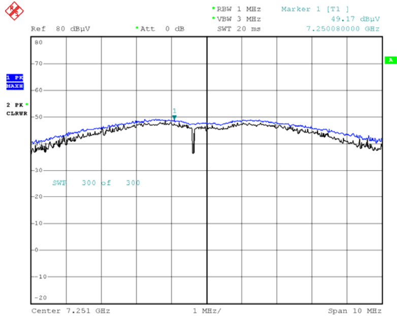
Radiated Spurious Emissions plot – Peak Reading (802.11b, Ch.2 3rd Harmonic)
