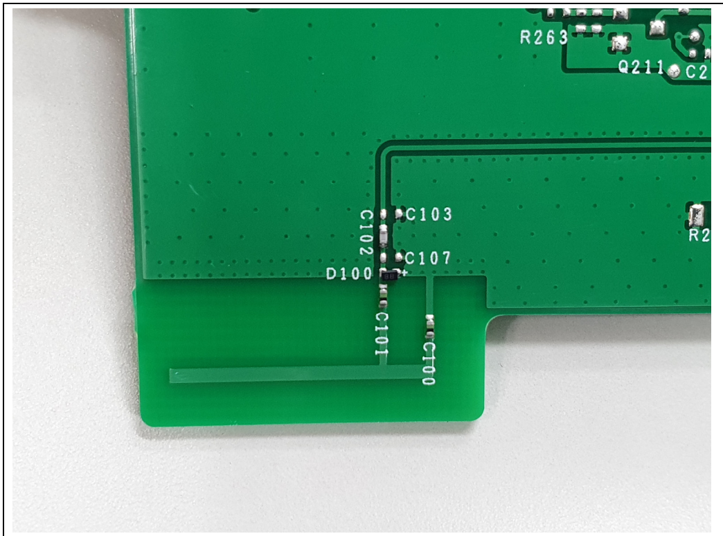
<BT Antenna>
