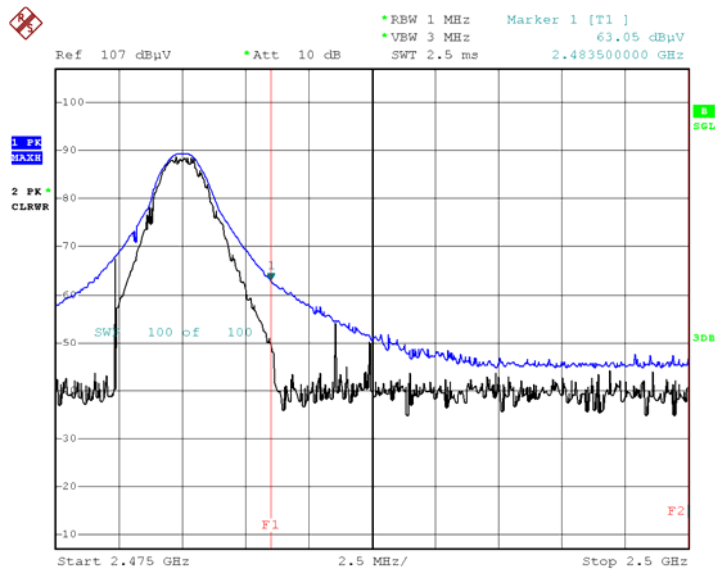
Radiated Restricted Band Edges plot – ( \pi/4 DQPSK, Ch.78, X-V)
