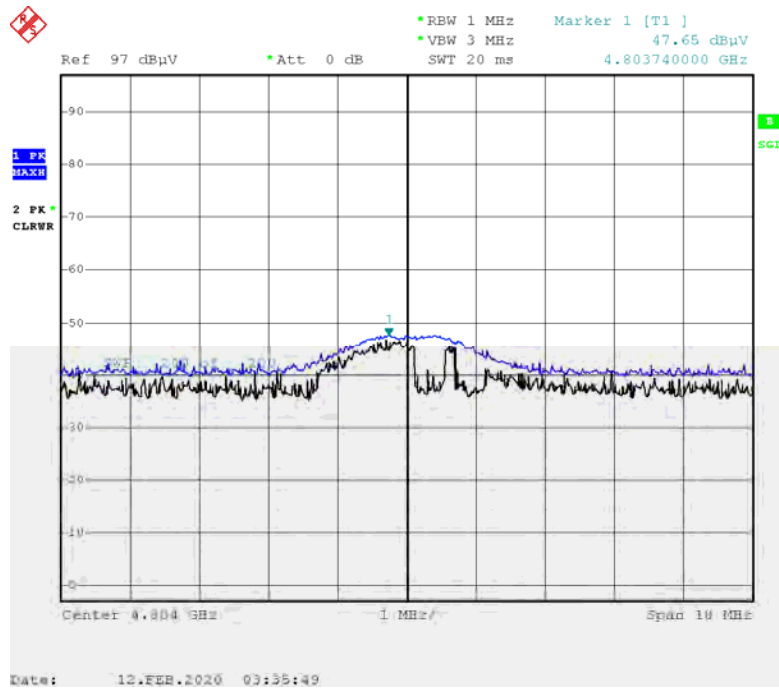
Radiated Spurious Emissions plot – Peak Reading (GFSK, Ch.0 2nd Harmonic, X-H)
