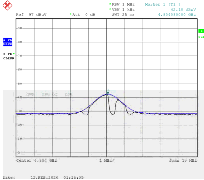
Radiated Spurious Emissions plot – Peak Reading (GFSK, Ch.0 2nd Harmonic, X-H)
