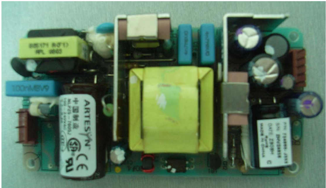
Internal of EUT-9
