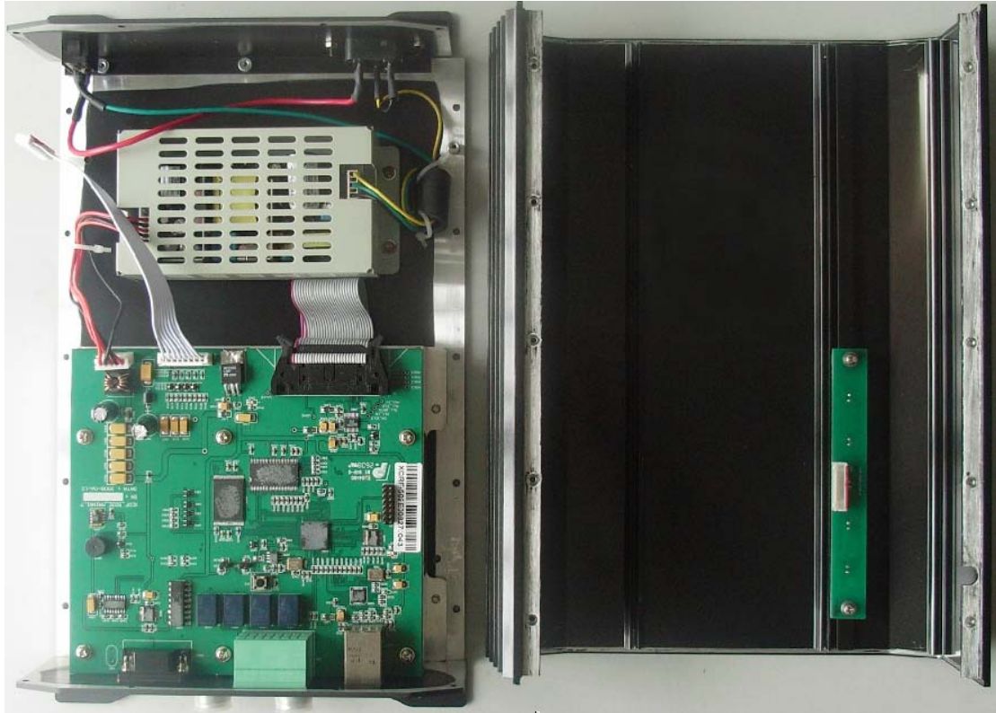
Internal of EUT-1
