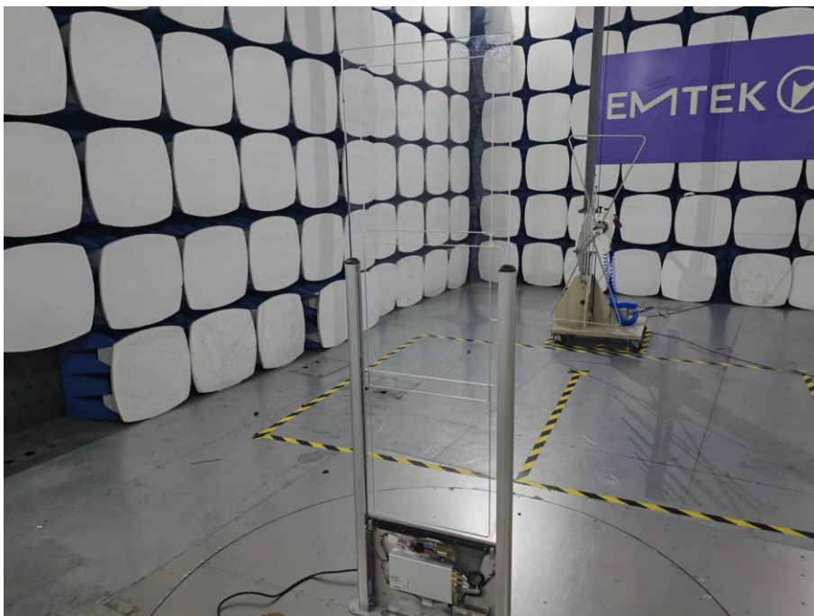
Spurious Emission Test Setup (Above 30MHz)
