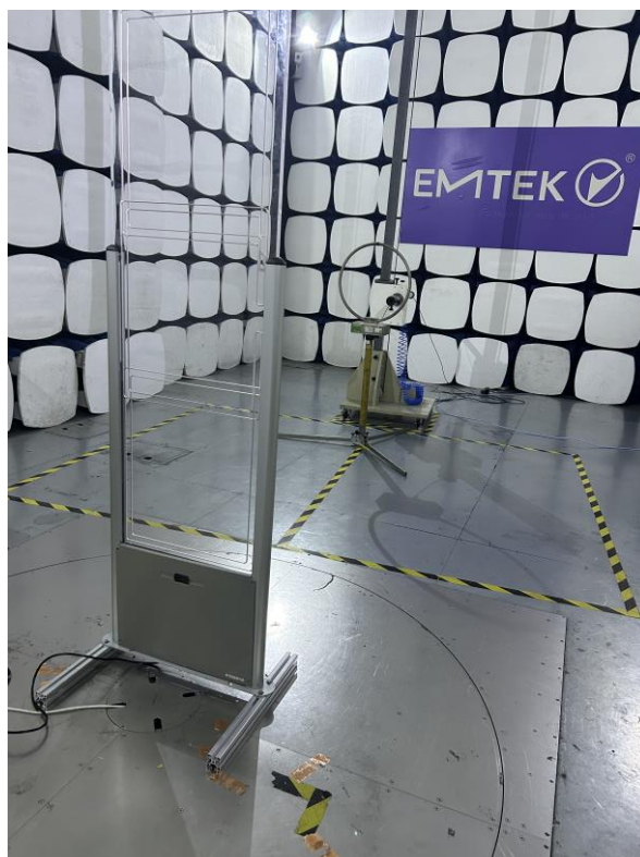
Spurious Emission Test Setup (Above 30MHz)
