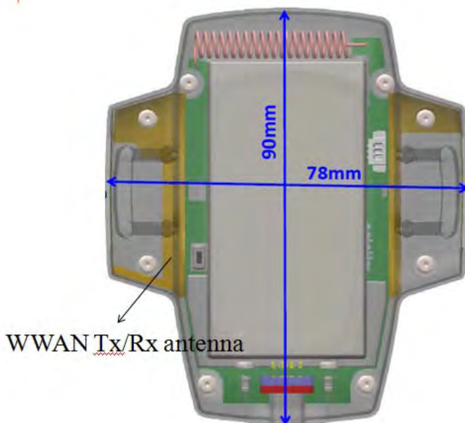
Fig.7 Antenna position plot (Back view)
