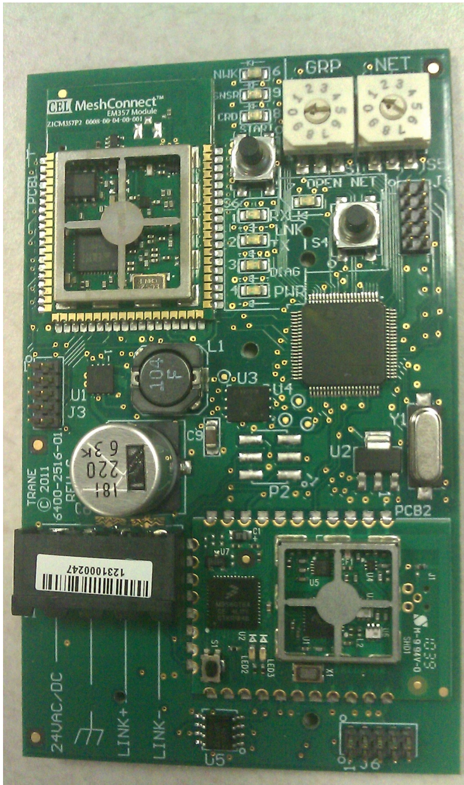
WCI Front PCBA with Shields Removed
