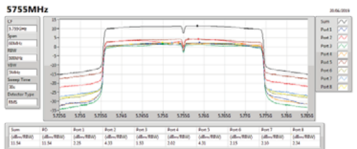
802.11ax HEW40_Nss1,(MCS0)_8TX
