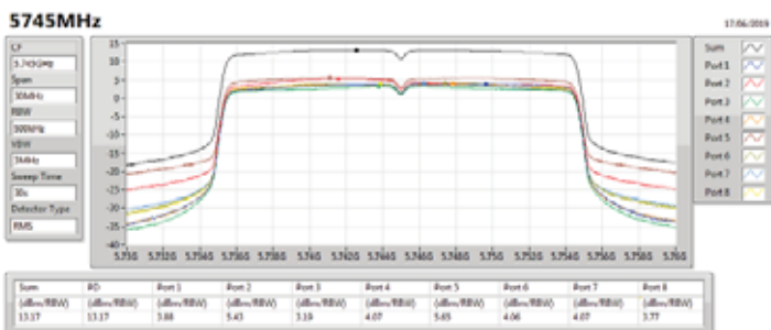
802.11ax HEW20_Nss1,(MCS0)_8TX
