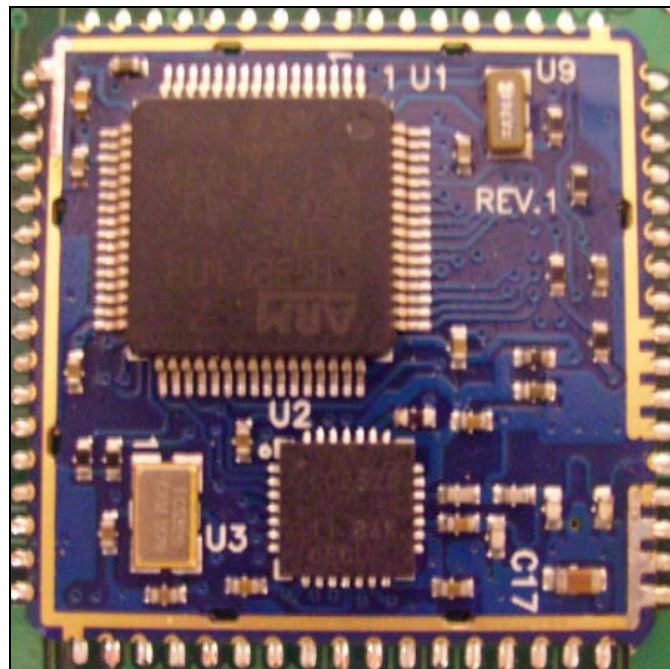
Photograph 4. EUT shield off
