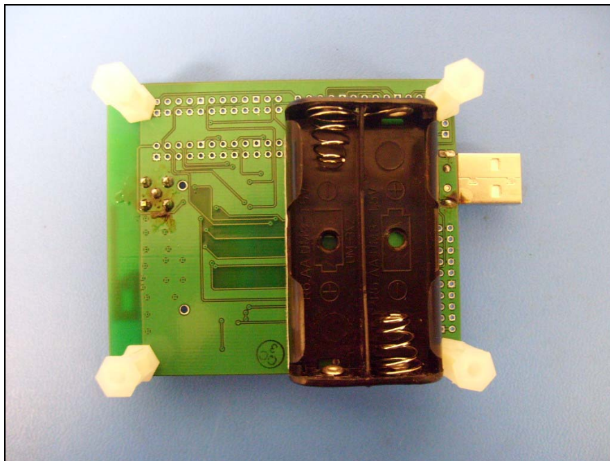
Photograph 2. Bottom View
