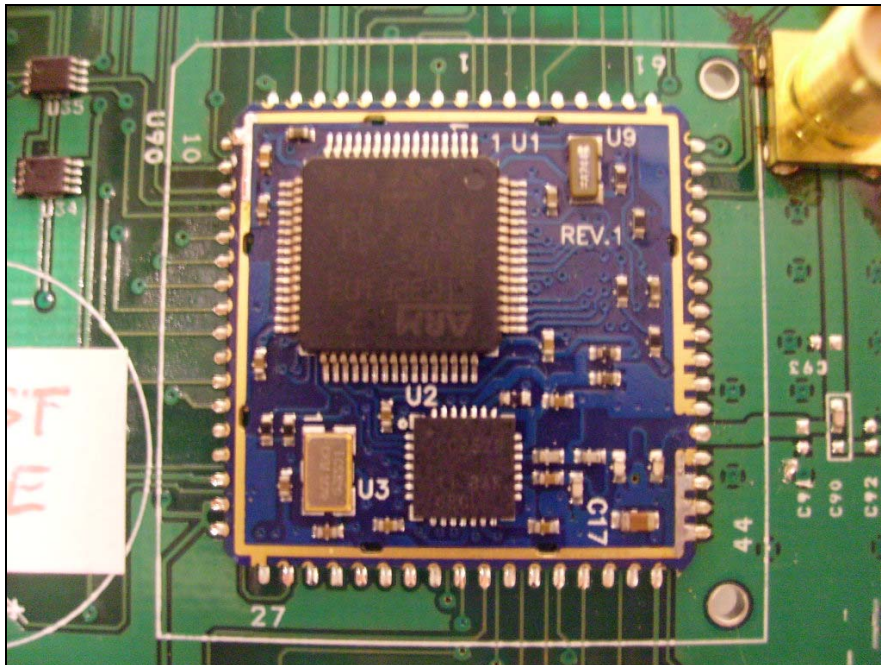
Photograph 7. Shield Off
