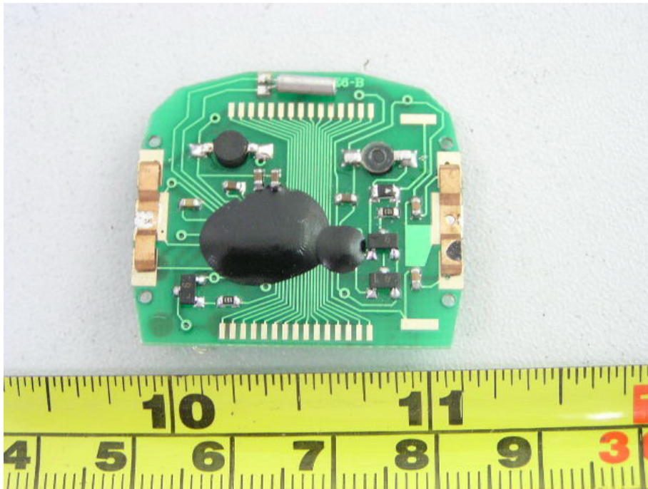
EUT – Bottom View of PCB View (1)
