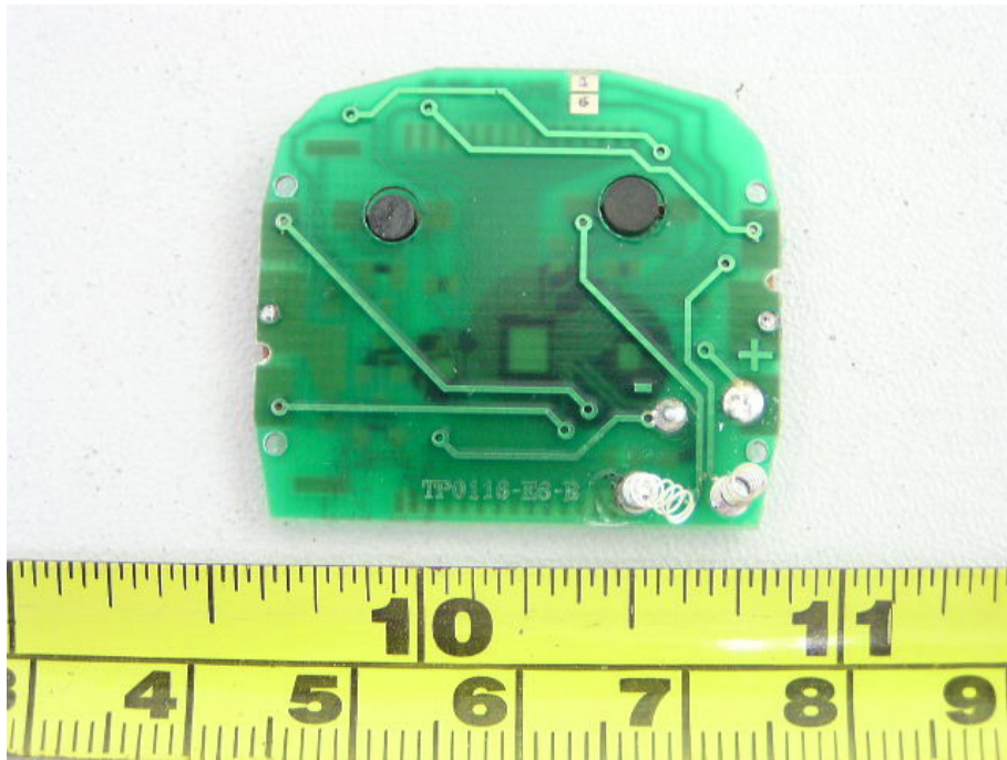
EUT – Top View of PCB View (1)
