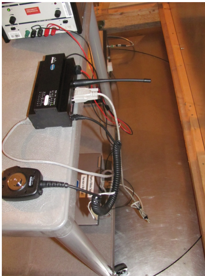
Conducted Emissions
