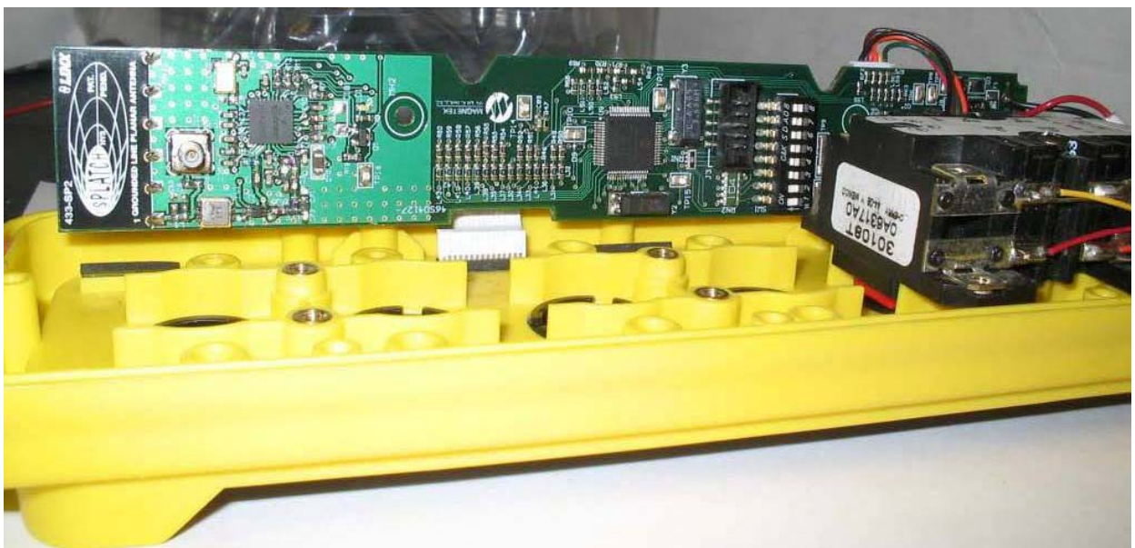
Board installed in Handheld Transmitter, Front View 2
