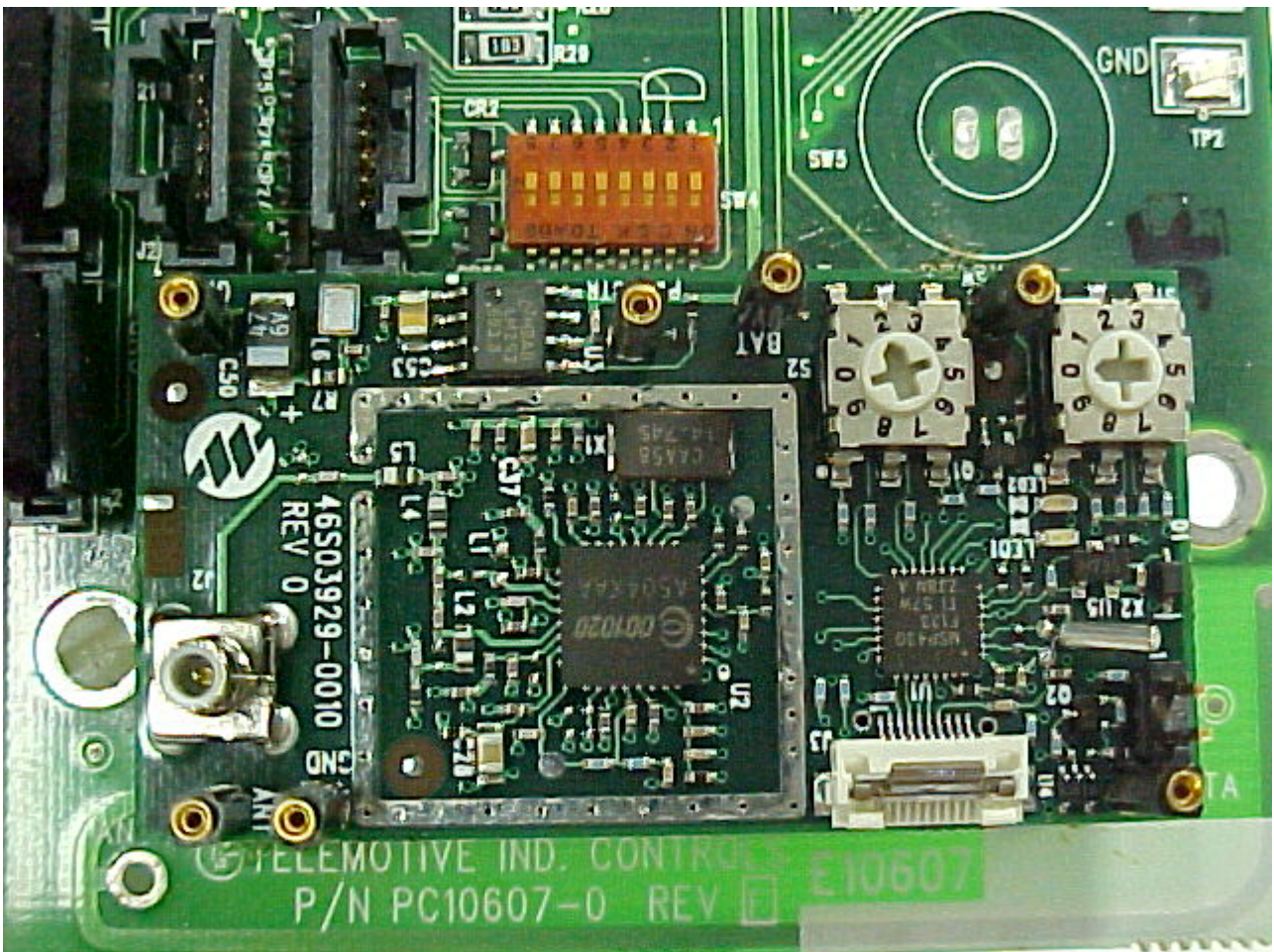
Photo Three – Internal Component Side of RF Board / Shielding Removed
