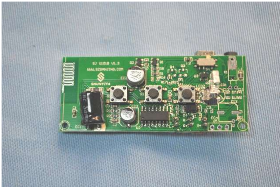
Main &amp; RF board component side
