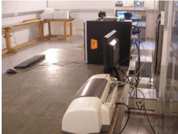
Radiated emission test view
